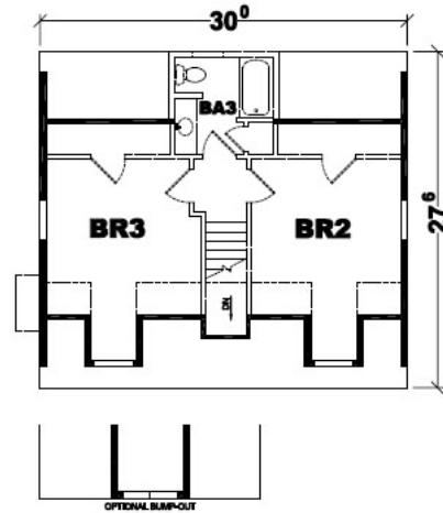
Proposed Second Floor Layout
