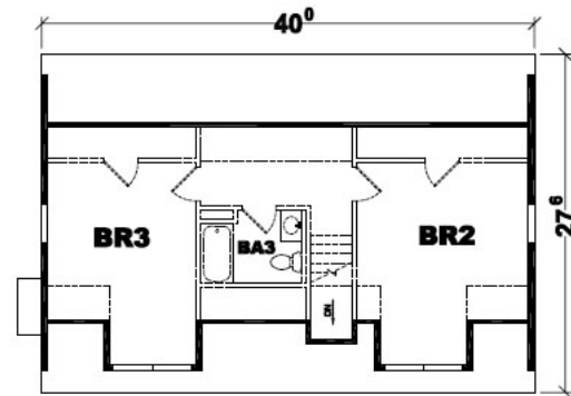
Proposed Second Floor Layout
