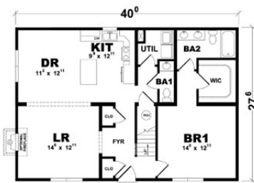
First Floor Layout
