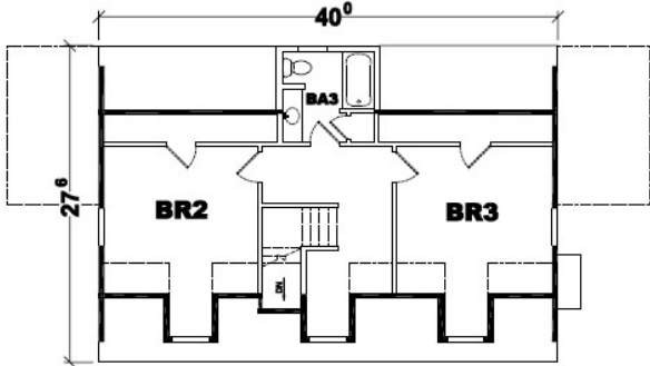
Proposed Second Floor Layout
