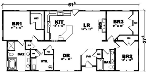
First Floor Layout
