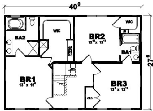
Second Floor Layout
